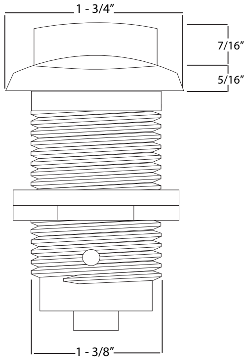
Assembly View
